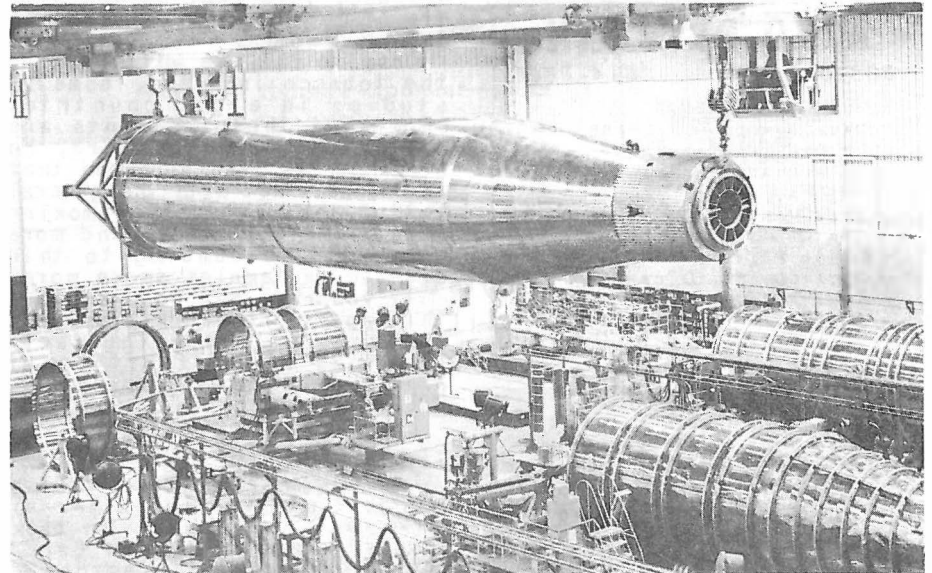
MOVING 10-TON HOOK IN MONORAIL CRANE 40 FEET ALOFT IS TICKLISH JOB FOR NELLIE KELLER. IN JUST ABOUT THE 'HIGHEST JOB' AT CONVAIR. MOVING THE GIANT ATLAS MISSILE. (CONVAIR PHOTO).
